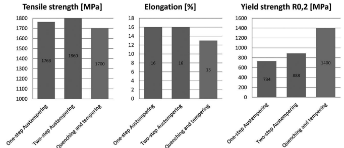
Fig. 10. Comparison of mechanical properties tested during static tensile tests
