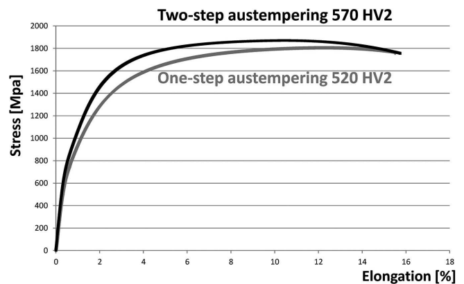
Fig. 11. Exemplary curves of extension. The green line – the one-step austempering and the black the two-step austempering
