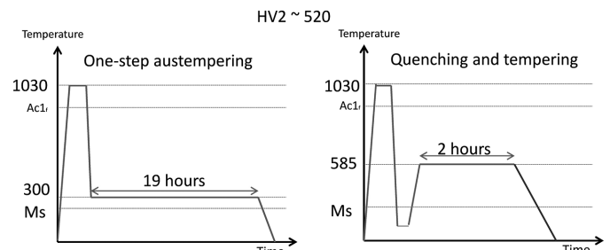
Fig. 2. Diagram applied heat treatments
