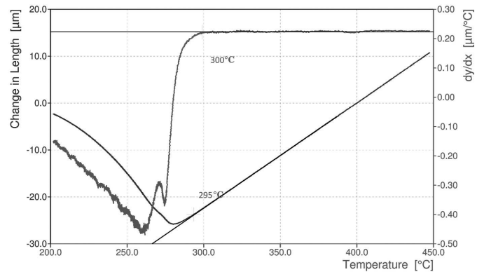
Fig. 1. Differential and dilatometric curve obtained during rapid cooling
